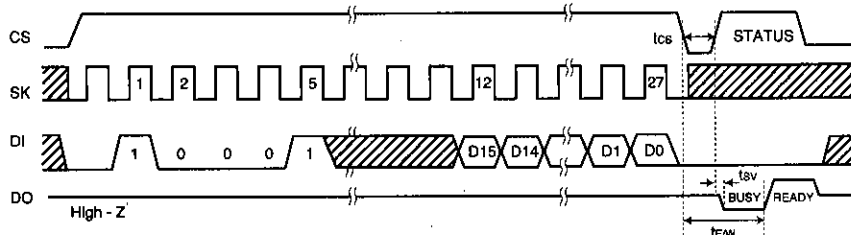
Fig. 5 All address write cycle timing
