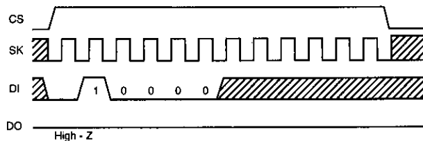
Fig. 6 Write disable cycle timing (WDS)
