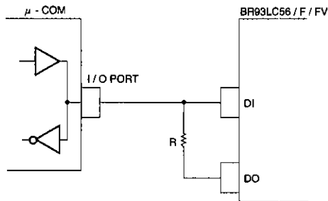
Fig. 11 Common connections for the DI and DO control line
