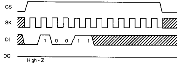
Fig. 3 Write enable cycle timing
