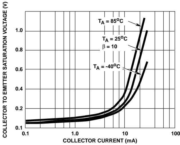
FIGURE 15. V_{CE SAT} (NPN) vs COLLECTOR CURRENT
