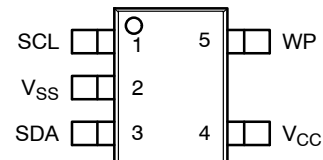
TSOT-23 (TD) (Top View)
