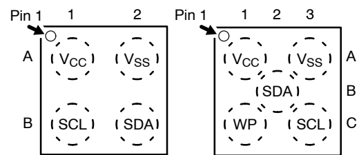
WLCSP-4** (Top Views) WLCSP-5** (Top Views)
