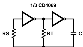
FOR TYPICAL COMPONENT VALUES AND CIRCUIT PERFORMANCE, SEE APPLICATION NOTE AN-6466 FIGURE 16. TYPICAL RC OSCILLATOR CIRCUIT
