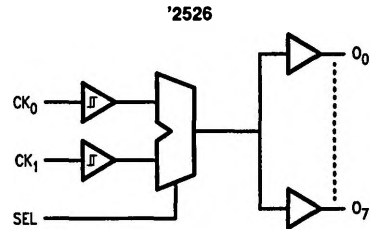
TL/F/10684-8
