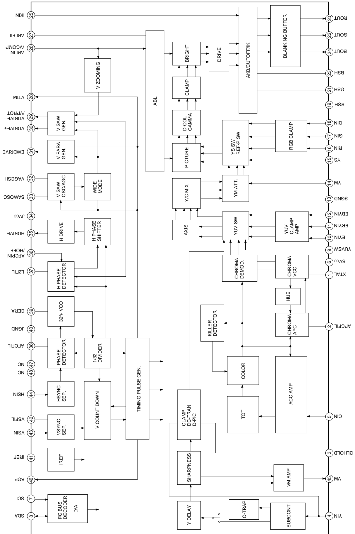
Block Diagram
