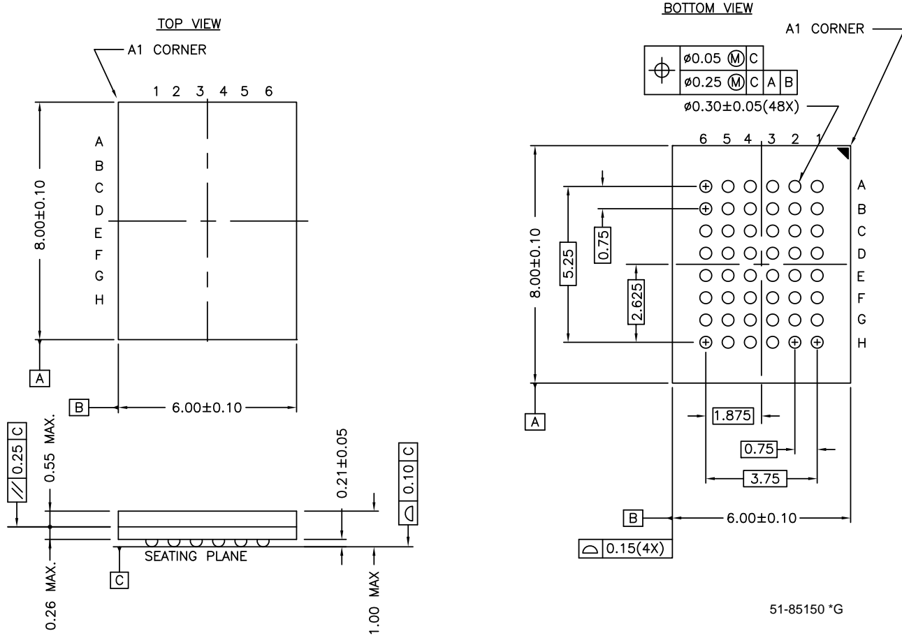
Figure 1. 48-ball VFBGA (6 × 8 × 1 mm) BV48/BZ48, 51-85150
