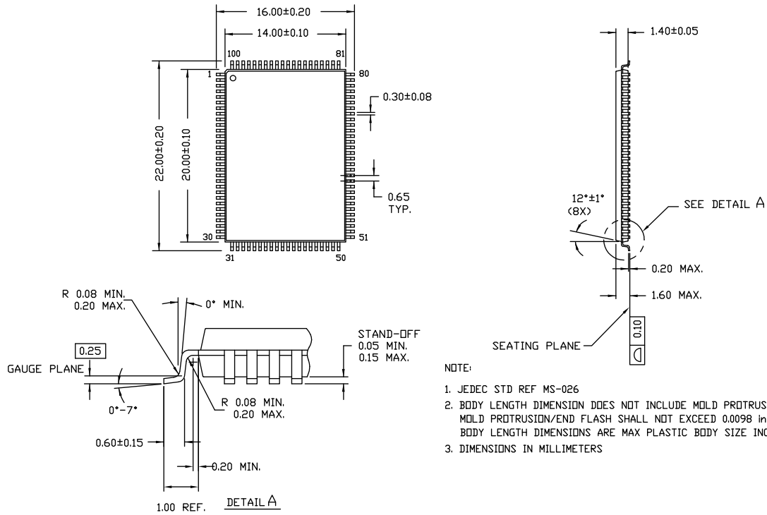
Figure 10. 100-pin TQFP (14 × 20 × 1.4 mm) A100RA Package Outline, 51-85050
