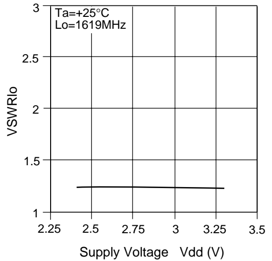
VSWR(Lo) vs. Supply Voltage
