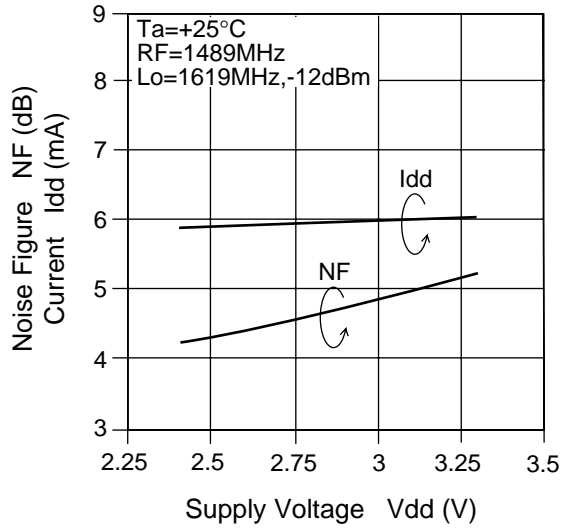
Noise Figure, Current vs. Supply Voltage
