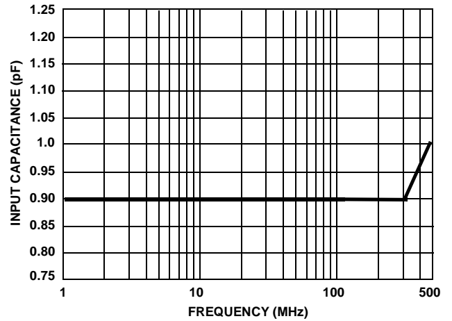
FIGURE 2. INPUT CAPACITANCE vs FREQUENCY
