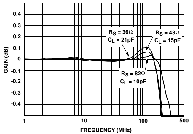
FIGURE 4. GAIN FLATNESS
