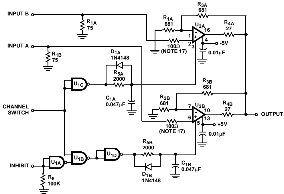
FIGURE 9. TWO CHANNEL HIGH IMPEDANCE MULTIPLEXER
