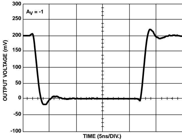
FIGURE 12. SMALL SIGNAL POSITIVE PULSE RESPONSE
