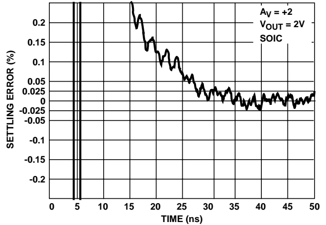
FIGURE 19. SETTLING RESPONSE
