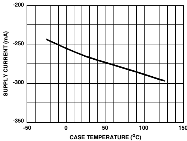
FIGURE 16. SUPPLY CURRENT vs TEMPERATURE CHARACTERISTICS
