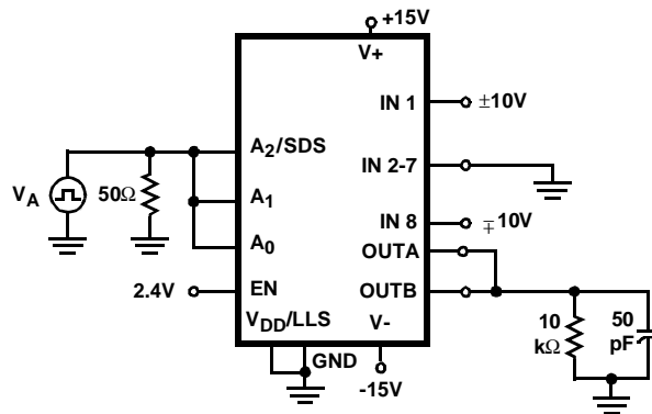
FIGURE 5B. TEST CIRCUIT
