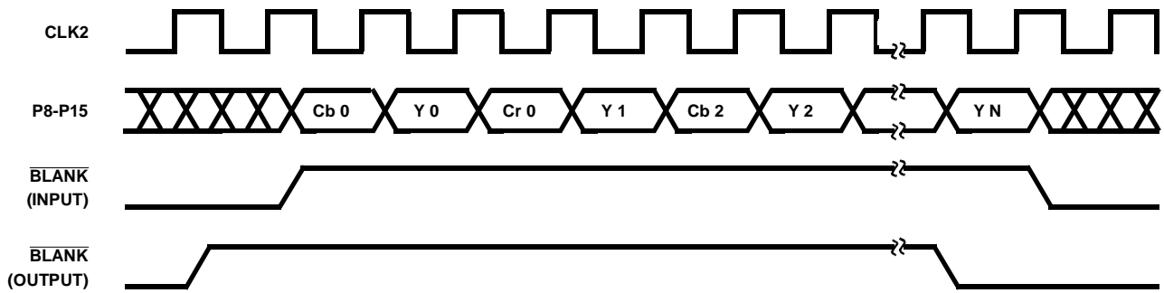
FIGURE 1. PIXEL INPUT TIMING - 8-BIT YCBCR
