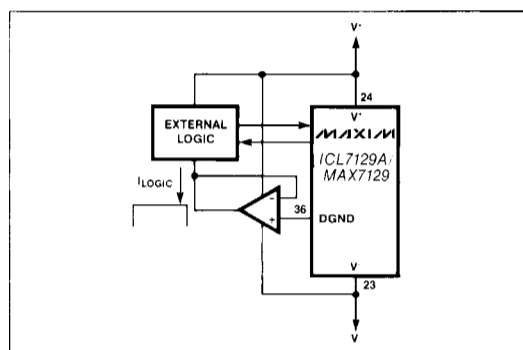
Figure 11. DGND Buffer
