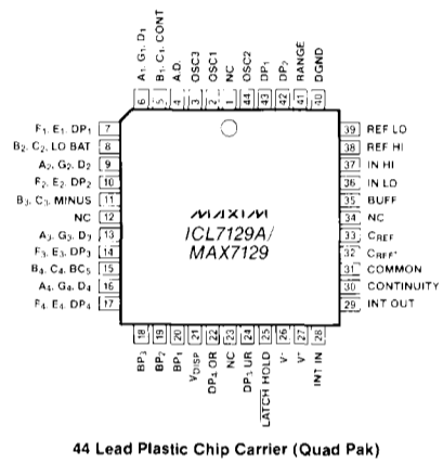
Pin Configuration
