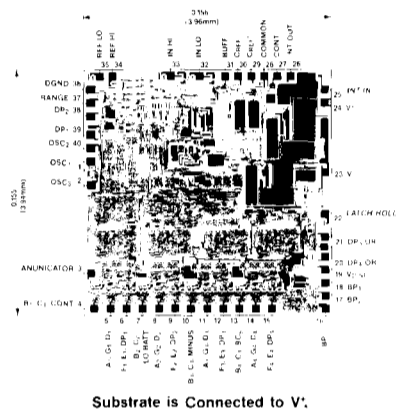
Chip Topography
