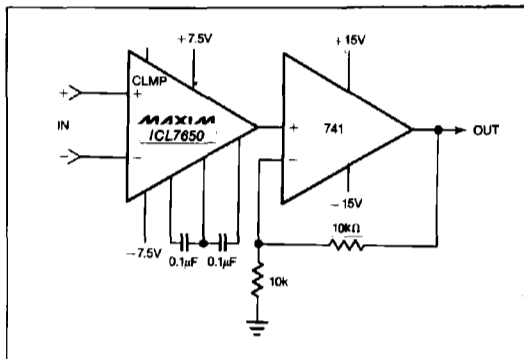
Figure 7. Using 741 to boost Output Drive Capability
