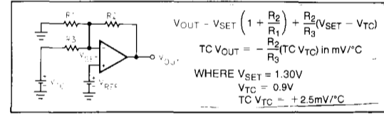
Figure 5. Maxim's Generation of Negative Temperature Coefficients.
