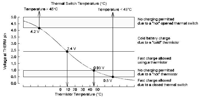
Figure 7: Voltage levels for temperature sensing with a thermistor or thermal switch
