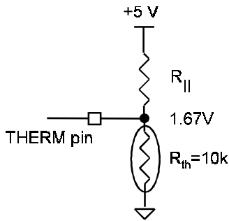
Figure 9: Equivalent voltage divider
