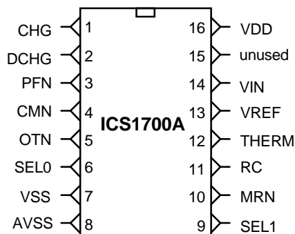
16-Pin DIP
