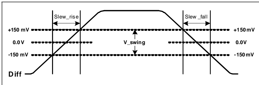
Figure 5. Differential Measurements
