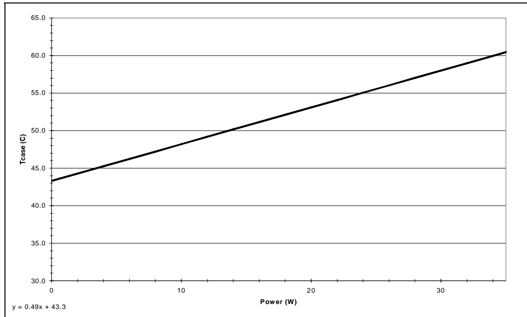
Figure 16. Thermal Profile
