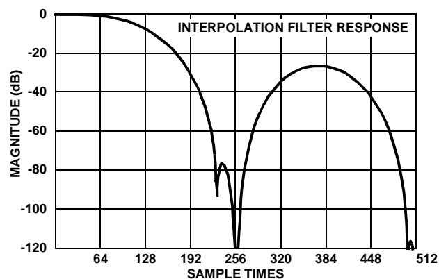
FIGURE 13B. INTERPOLATION FILTER IMPULSE RESPONSE L = 16; FOUT = 4096
