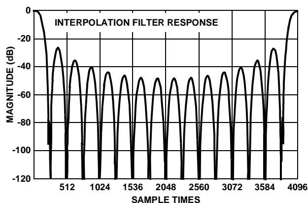
FIGURE 13A. INTERPOLATION FILTER IMPULSE RESPONSE L = 16; FOUT = 4096
