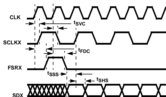
FIGURE 20. SERIAL INTERFACE RELATIVE TIMING
