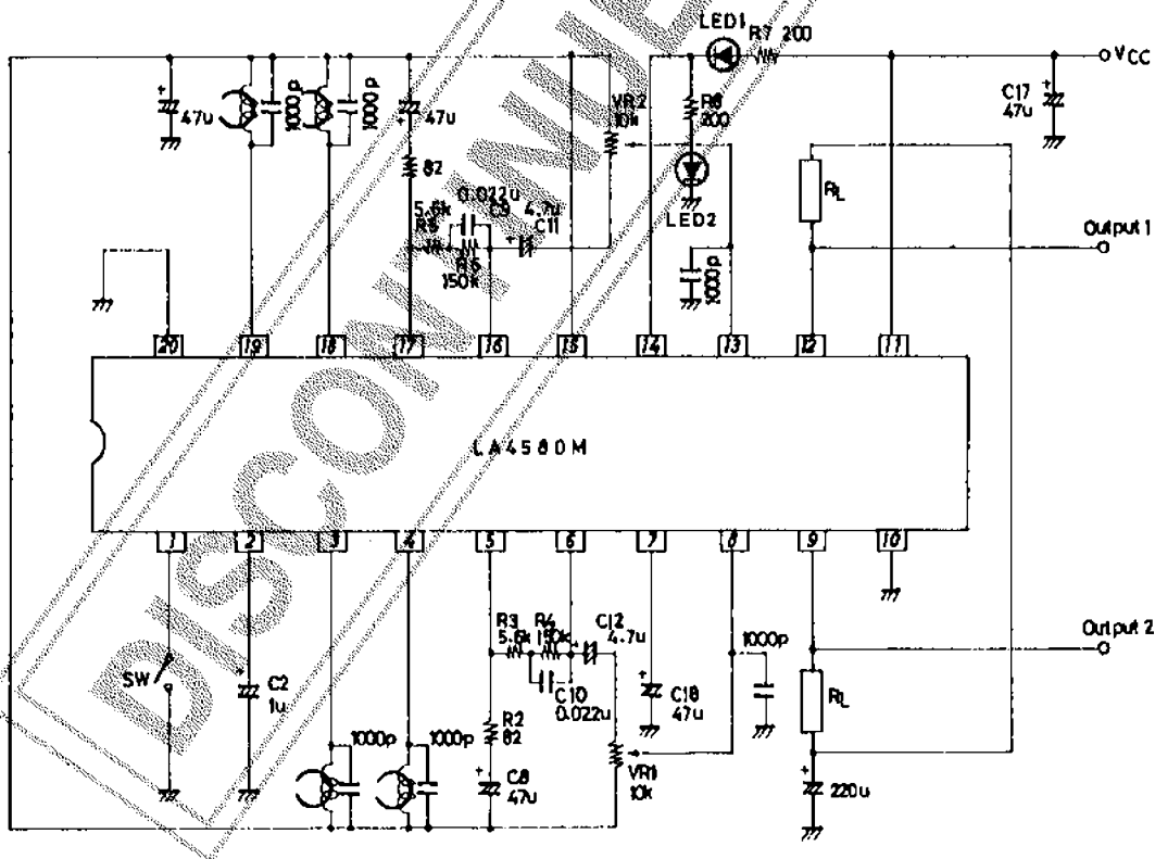
Sample Application Circuit (2): Power output capacitor common method
