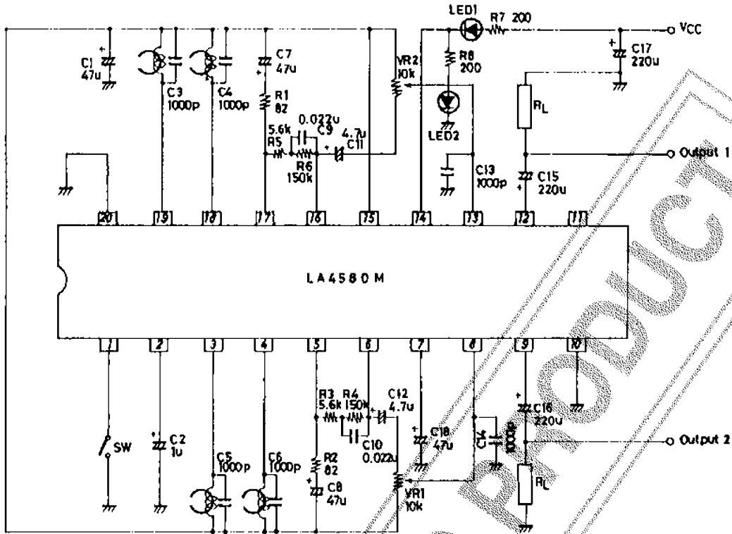
Sample Application Circuit (1): Power input capacitor method
