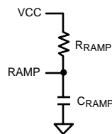
Figure 7. R_{\text{RAMP}} to V_{\text{CC}} for V_{\text{OUT}} > 7.5\text{V}
