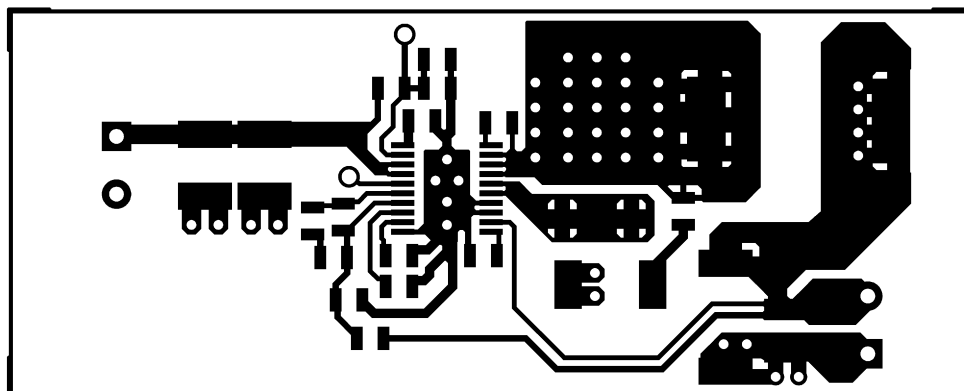
Figure 14. Component Side
