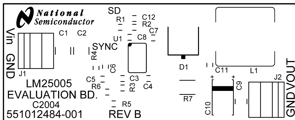
Figure 16. Silkscreen
