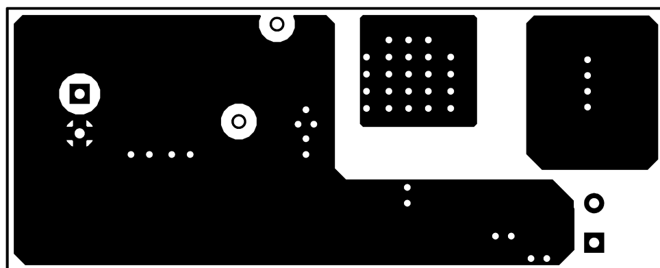
Figure 15. Solder Side
