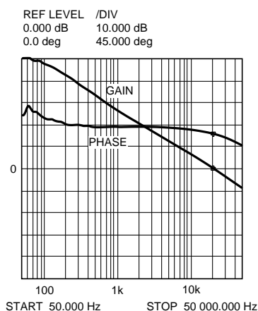
Figure 11. Overall Loop Gain and Phase
