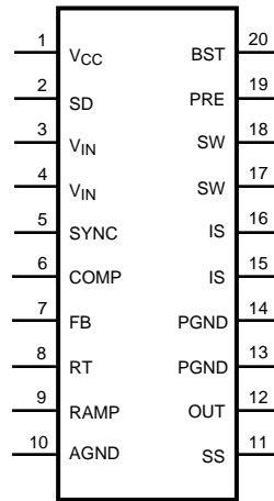
Figure 1. Top View 20-Lead TSSOP
