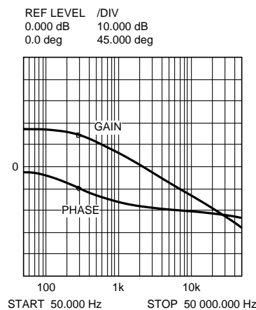
Figure 9. Gain and Phase of Modulator R_{\text{LOAD}} = 5 \text{ Ohms} and C_{\text{OUT}} = 177 \mu\text{F}
