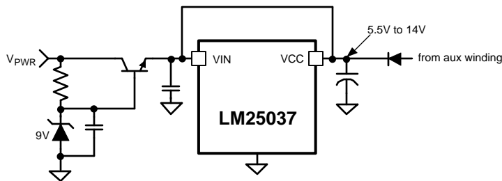
Figure 24. Start-up Regulator for VPWR >75V
