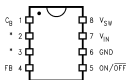
Figure 2. SO-8/DIP Package 8-Lead Package Top View
