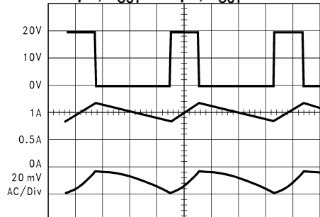
Figure 3. Horizontal Time Base: 1 \mu s /div
