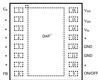
Figure 1. 16-Lead LLP Surface Mount Package Top View
