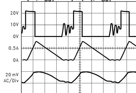
Figure 4. Horizontal Time Base: 1 \mu s /div
