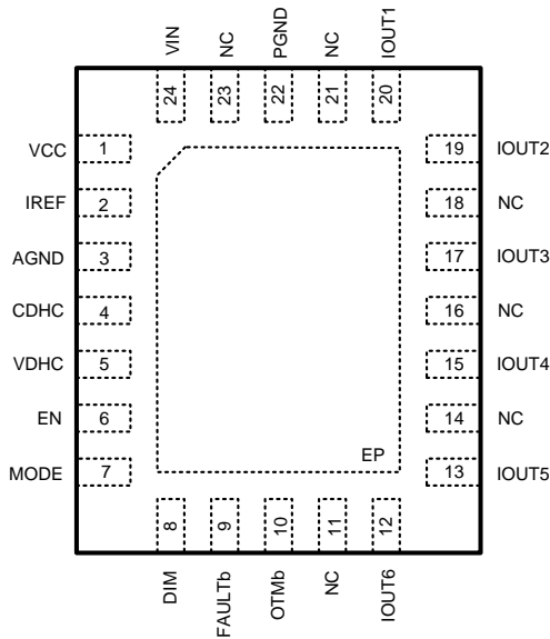
Figure 1. Top View 24 Lead Plastic WQFN-24
