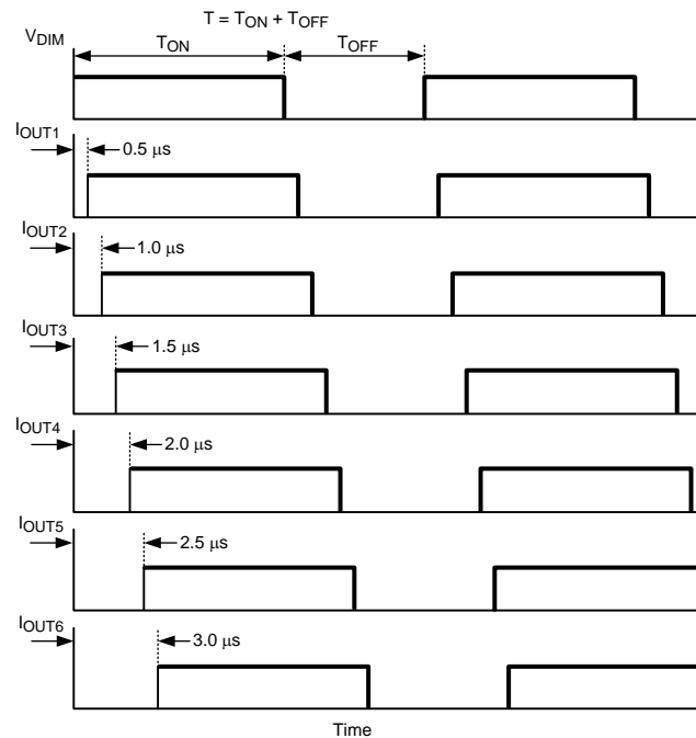
Figure 15. PWM Dimming Switching Timing
