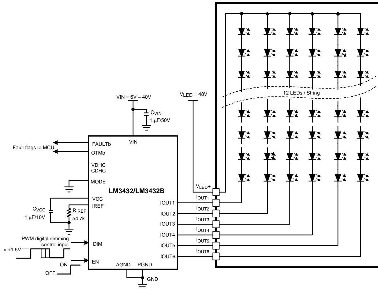
Figure 17. Typical Application Schematic to Drive 72 White LEDs (@20 mA) (PWM Digital Dimming)
