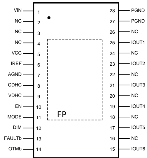
Figure 2. Top View 28 Lead Plastic eHTSSOP-28
