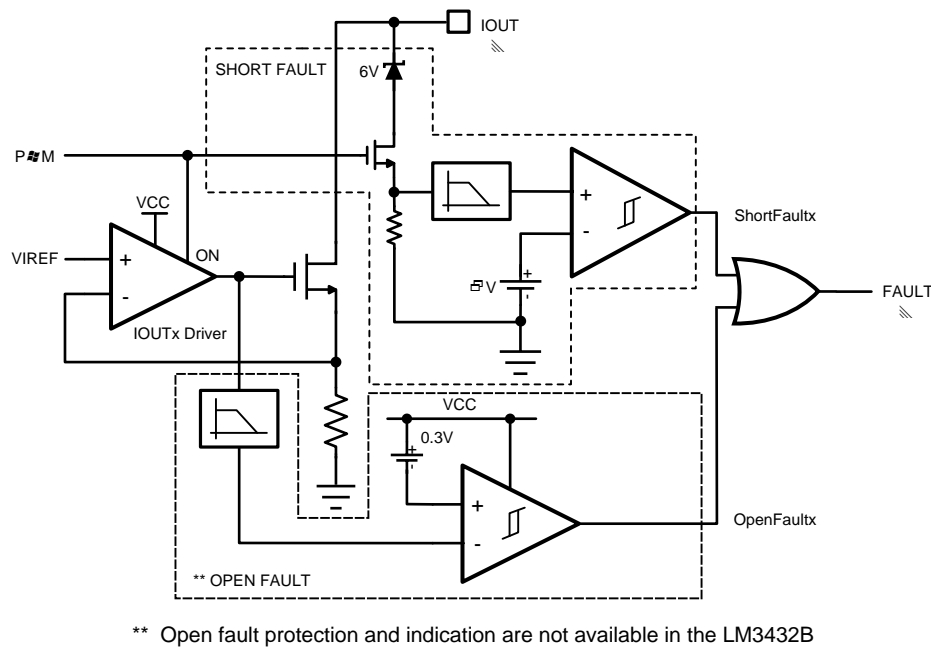
Figure 16. Fault Detect Functional Block Diagram
