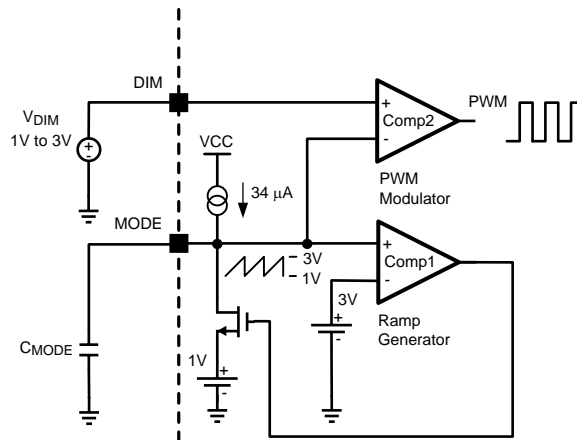
Figure 14. Analog Dimming of LEDs
