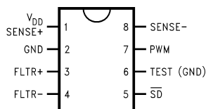
Figure 1. Top View LM3822 for High-Side Sensing
