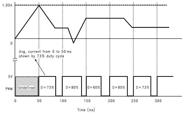
Figure 7. Typical Timing Diagram for Mostly Positive Current
