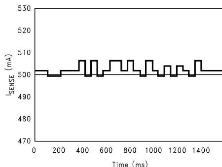
Figure 6. Typical Response of LM3822
