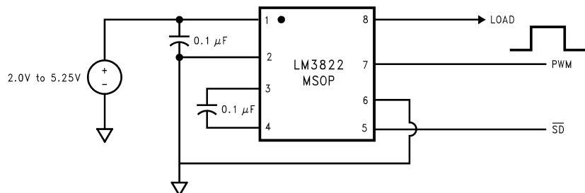
Figure 2. High Side Sense
