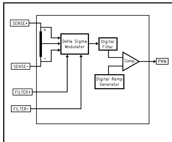
Figure 5. Functional block diagram of LM3822
