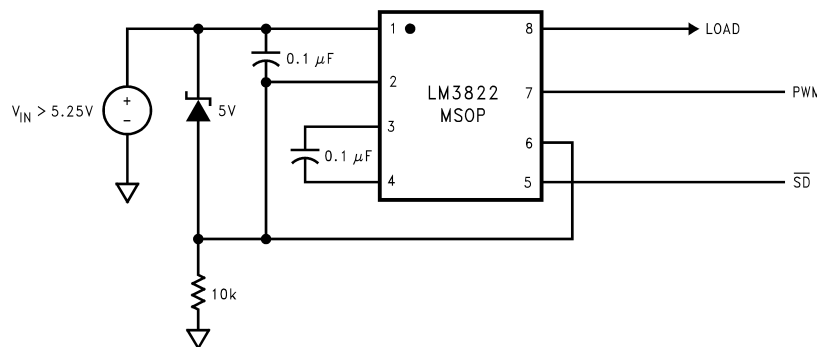
Figure 4. High Voltage Operation — V_{\text{IN}} Greater Than 5.5V (High Side Sense) (PWM output is referred to Pin 6)
