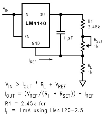
Figure 33. Precision Programmable Current Source
