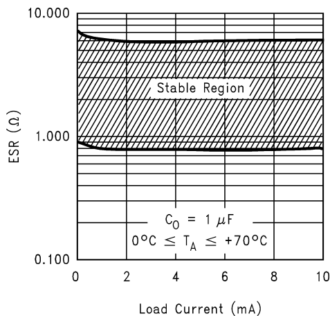
Figure 25. 1 \mu F ESR Range
