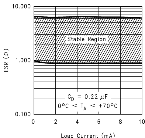
Figure 24. 0.22 \mu F ESR Range
