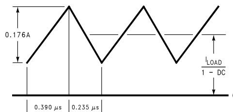
Figure 42. 10 \mu H Inductor Current 5V - 12V Boost (LM4805)
