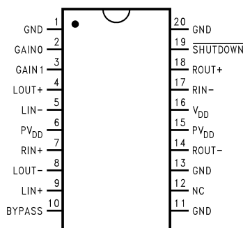
Figure 1. Top View
