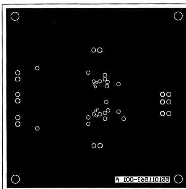
Figure 48. Recommended MH PC Board Layout: Bottom-Side Layout
