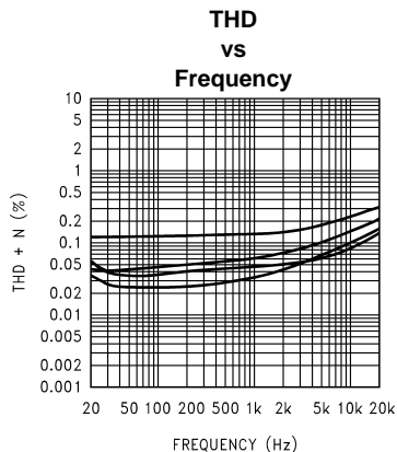
Figure 19. V_{DD} = 3\text{V} , R_L = 4\Omega , P_{OUT} = 150\text{mW} , at (from top to bottom at 1kHz): A_V = 21.6\text{dB} , A_V = 15.6\text{dB} , A_V = 10\text{dB} , A_V = 6\text{dB}
