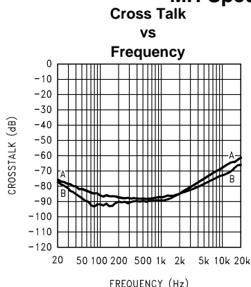
Figure 39. V_{DD} = 5V , R_L = 8\Omega , A_V = 21.6dB , A = Left channel driven, right channel measured; B = Right channel driven, left channel measured
