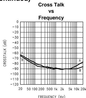
Figure 40. V_{DD} = 3V , R_L = 8\Omega , A_V = 6dB , A = Left channel driven, right channel measured; B = Right channel driven, left channel measured
