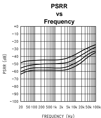
Figure 17. V_{DD} = 5\text{V} , R_L = 4\Omega , R_{SOURCE} = 10\Omega , V_{RIPPLE} = 200\text{mV}_{P-P} , at (from top to bottom at 1kHz): A_V = 21.6\text{dB} , A_V = 15.6\text{dB} , A_V = 10\text{dB} , A_V = 6\text{dB}
