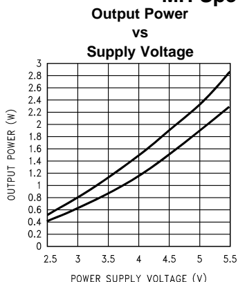
Figure 15. R_L = 4\Omega , f_{IN} = 1\text{kHz} , at (from top to bottom at 4V): THD+N = 10%, THD+N = 1%
