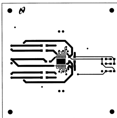
Figure 45. Recommended MH PC Board Layout: Component-Side Layout
