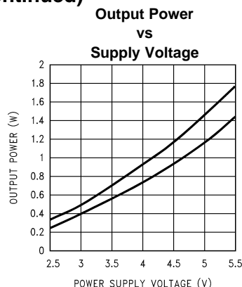
Figure 16. R_L = 8\Omega , f_{IN} = 1\text{kHz} , at (from top to bottom at 4V): THD+N = 10%, THD+N = 1%
