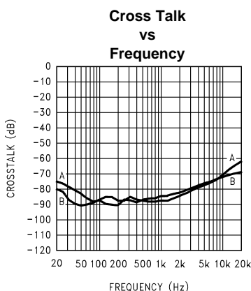
Figure 43. V_{DD} = 3V , R_L = 8\Omega , A_V = 21.6dB , A = Left channel driven, right channel measured; B = Right channel driven, left channel measured
