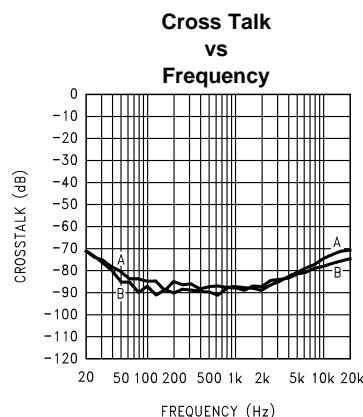
Figure 42. V_{DD} = 3V , R_L = 8\Omega , A_V = 15.6dB , A = Left channel driven, right channel measured; B = Right channel driven, left channel measured
