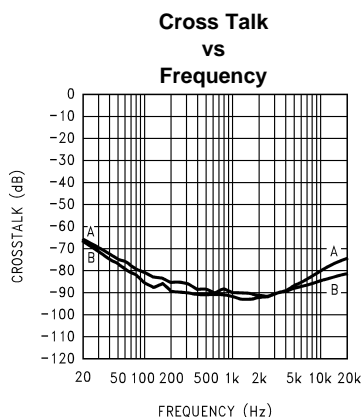
Figure 41. V_{DD} = 3V , R_L = 8\Omega , A_V = 10dB , A = Left channel driven, right channel measured; B = Right channel driven, left channel measured
