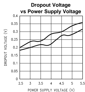
Figure 32. R_L = 8\Omega , f_{IN} = 1kHz , both channels driven and loaded at (from top to bottom at 4V): positive signal swing, negative signal swing
