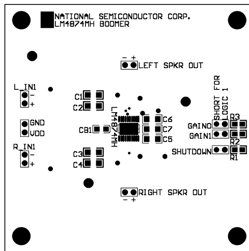
Figure 44. Recommended MH PC Board Layout: Component-Side Silkscreen
