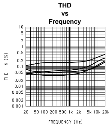
Figure 20. V_{DD} = 3\text{V} , R_L = 8\Omega , P_{OUT} = 150\text{mW} , at (from top to bottom at 1kHz): A_V = 21.6\text{dB} , A_V = 15.6\text{dB} , A_V = 10\text{dB} , A_V = 6\text{dB}
