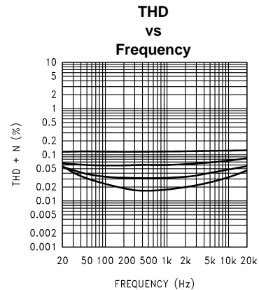
Figure 4. V_{DD} = 5V , R_L = 8\Omega , P_{OUT} = 400mW , at (from top to bottom at 1kHz): A_V = 21.6dB , A_V = 15.6dB , A_V = 10dB , A_V = 6dB
