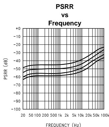
Figure 18. V_{DD} = 5\text{V} , R_L = 8\Omega , R_{SOURCE} = 10\Omega , V_{RIPPLE} = 200\text{mV}_{P-P} , at (from top to bottom at 1kHz): A_V = 21.6\text{dB} , A_V = 15.6\text{dB} , A_V = 10\text{dB} , A_V = 6\text{dB}
