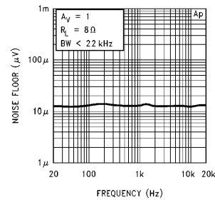
Noise Floor
