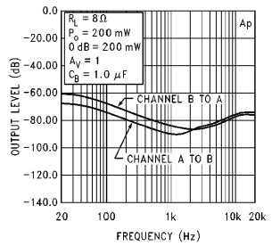
Channel Separation
