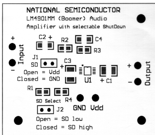
Figure 15. Silk Screen
