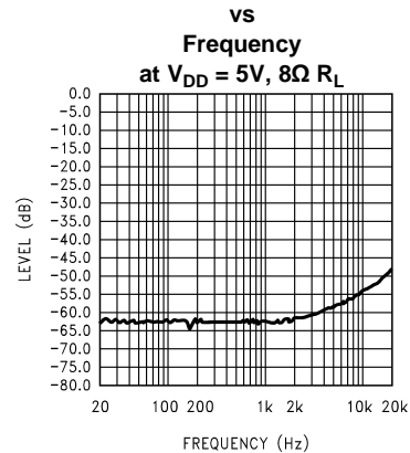
Figure 7. Input Floating
