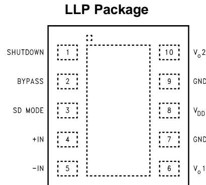
Figure 4. Top View Order Number LM4901LD See NS Package Number LDA10B
