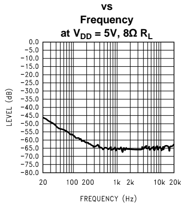
Figure 6. Input terminated with 10\Omega
