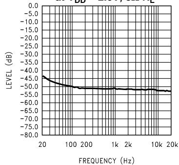
Figure 10. Input terminated with 10\Omega
