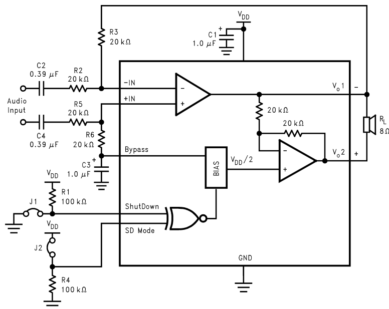
Figure 13. DIFFERENTIAL AMPLIFIER CONFIGURATION FOR LM4901
