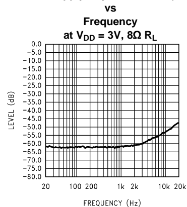
Figure 9. Input Floating
