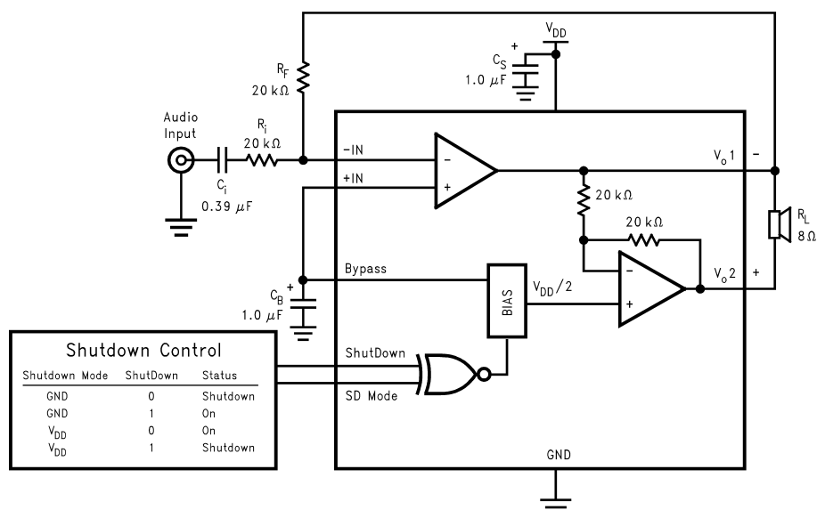
Figure 1. Typical Audio Amplifier Application Circuit
