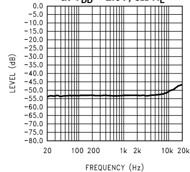
Figure 11. Input Floating
