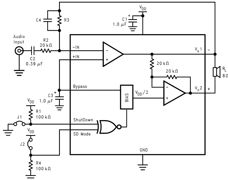
Figure 12. HIGHER GAIN AUDIO AMPLIFIER
