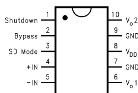
Figure 2. Top View Order Number LM4901MM See NS Package Number MUB10A
