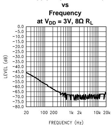
Figure 8. Input terminated with 10\Omega
