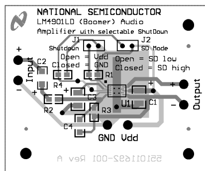
Figure 18. Composite View
