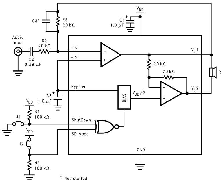
Figure 14. REFERENCE DESIGN BOARD SCHEMATIC
