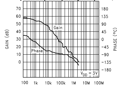
Figure 11. Input Floating
