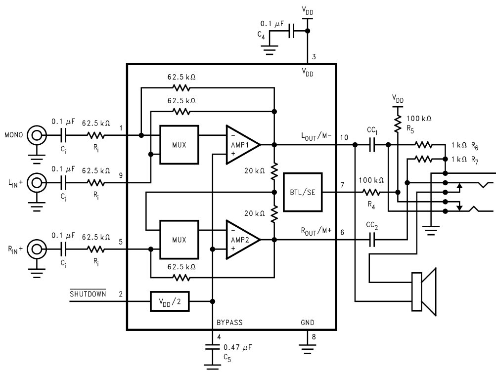
Figure 2. Typical Audio Amplifier Application Circuit
