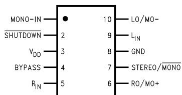
Figure 1. Top View
