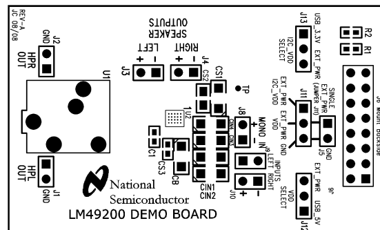
Figure 37. Silk Screen
