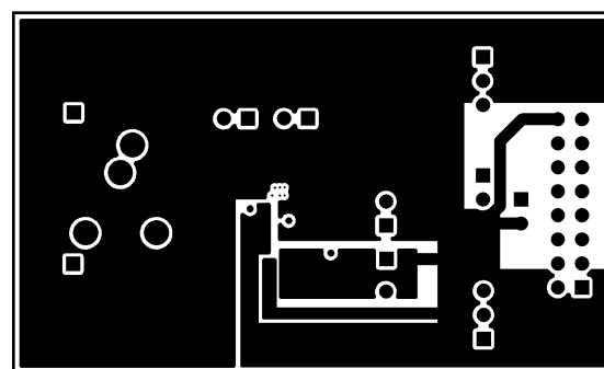
Figure 39. Internal Layer 1
