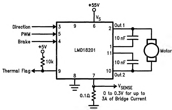
Current Sensing
