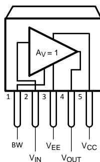
Figure 2. Top View TO-263 Package (Note 9)
