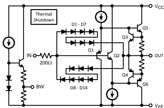
Figure 6. Simplified Circuit Diagram
