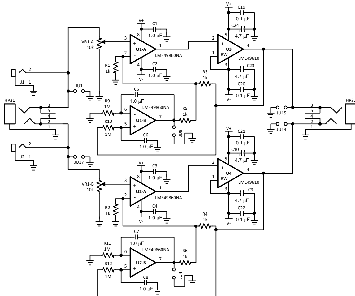
Figure 5. LME49610 delivers high output current for this high performance headphone amplifier
