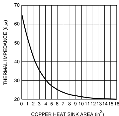
Figure 8. Thermal Resistance (typ) for 5 lead TO-263 Package Mounted on 1oz. copper
