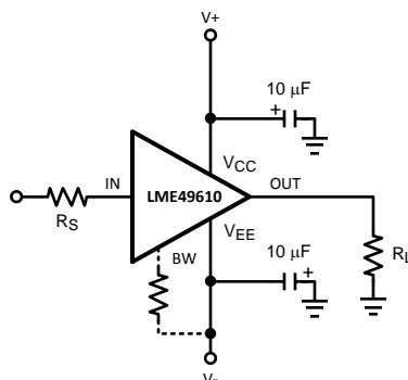
Figure 7. Buffer Connections
