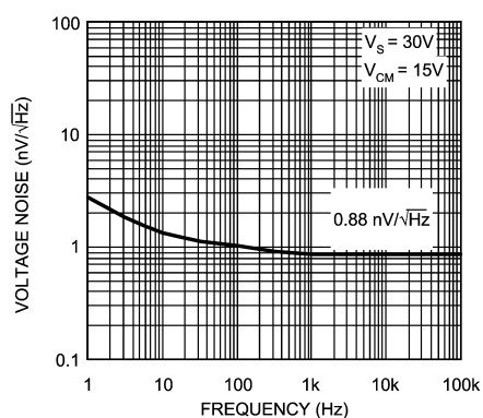
Figure 1. FIGURE 1: Voltage Noise Spectral Density
