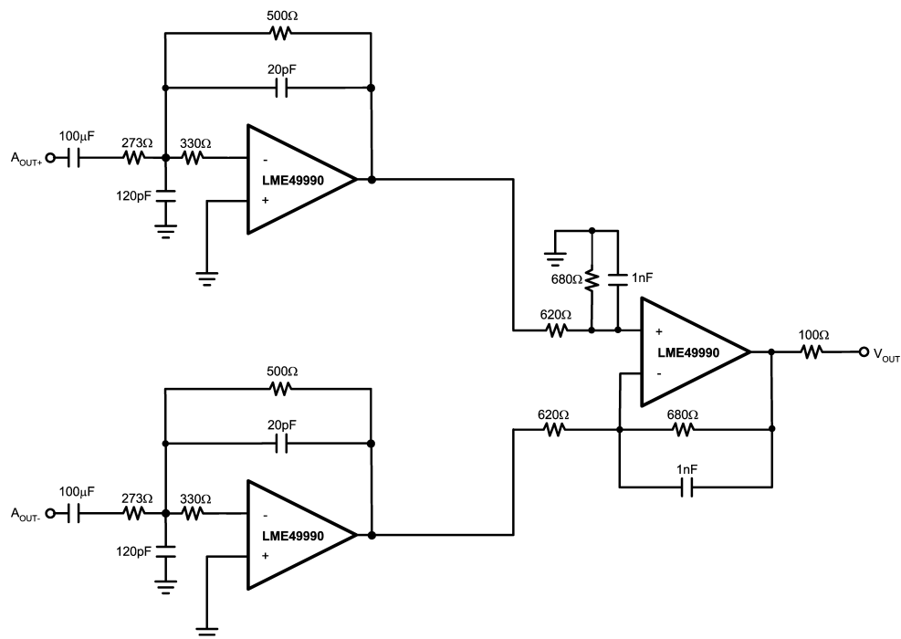
Figure 8. MFB 3rd Order PCM LPF
