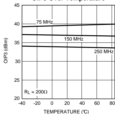
OIP3 Over Temperature
