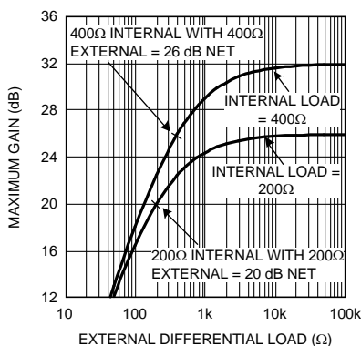
Figure 6. Gain vs. External Load
