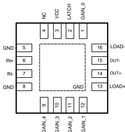
Figure 1. 16-Pin LLP (Top View)
