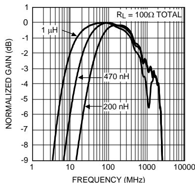
Figure 5. Bandwidth Changes Due to Different Inductor Values
