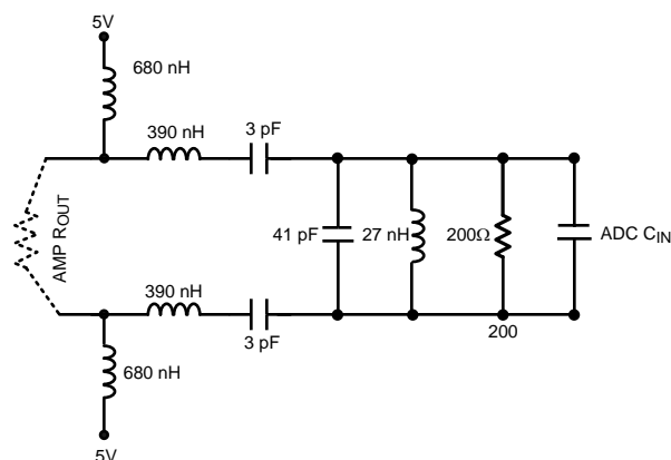
Figure 7. Bandpass Filter Center Frequency is 140 MHz with a 20 MHz Bandwidth Designed for 200 \Omega Impedance
