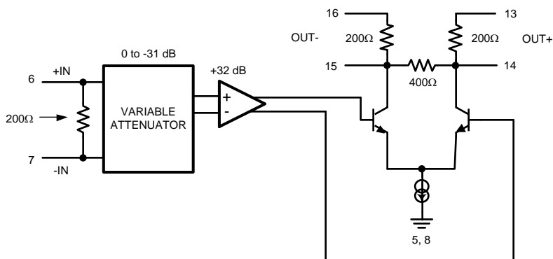
Figure 3. LMH6515 Block Diagram
