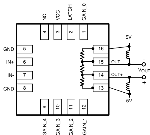
Figure 11. Using Low Gain Mode (200Ω Load)
