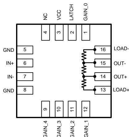
Figure 9. Internal Load Resistors
