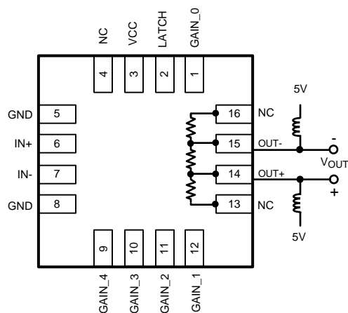
Figure 10. Using High Gain Mode (400Ω Load)
