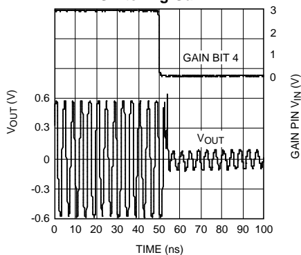
4 dB Gain Step Using Latch Pin
