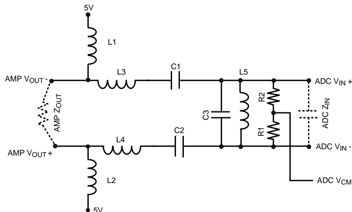
Figure 8. Sample Filter
