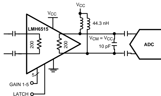
Figure 2. LMH6515 Typical Application
