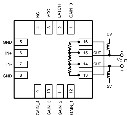
Figure 12. Alternate Connection for Low Gain Mode (200Ω Load)
