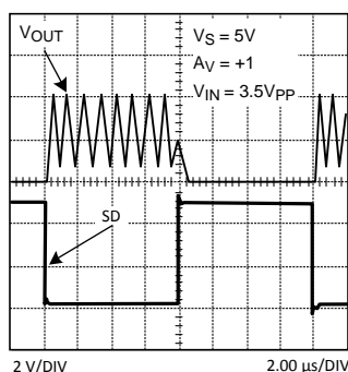
Figure 6. Output Held Low by Active Pull-Down Circuit
