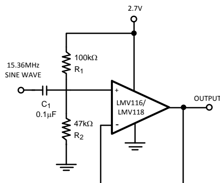
Figure 1. Non-Inverting Clock Buffer Amplifier
