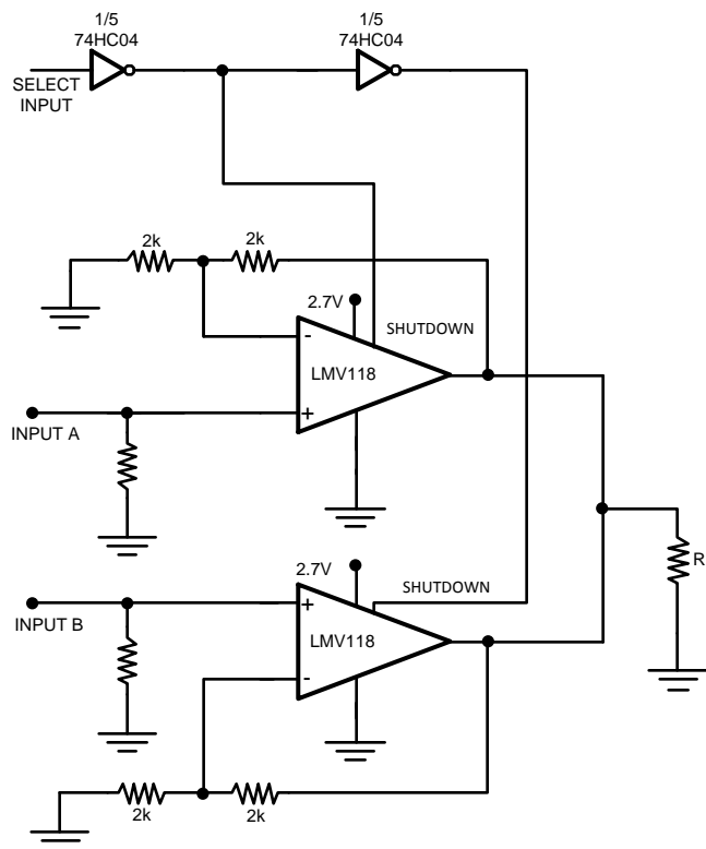
Figure 7. 2:1 MUX Operating off a 2.7V Single Supply
