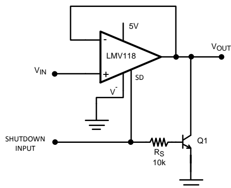
Figure 5. Active Pull-Down Schematic
