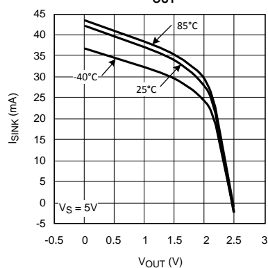
Sink Current vs. VOUT
