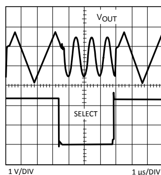
Figure 8. 2:1 MUX Output
