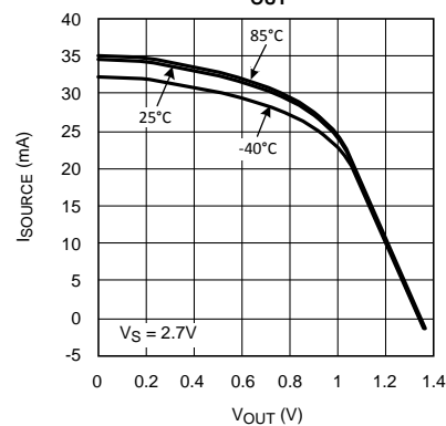
Source Current vs. VOUT
