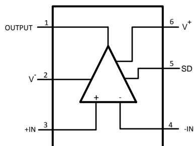
Figure 3. Top View
