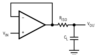
Figure 5. Isolation of C_L to Improve Stability
