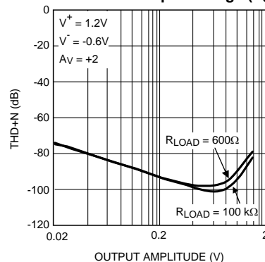
THD+N
