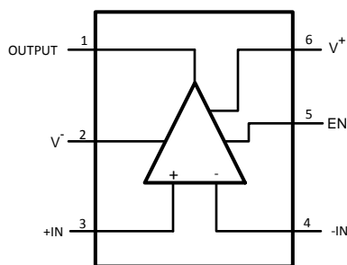
Figure 3. 6-Pin TSOT23 - Top View
