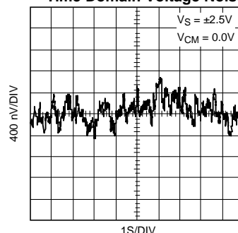
Time Domain Voltage Noise
