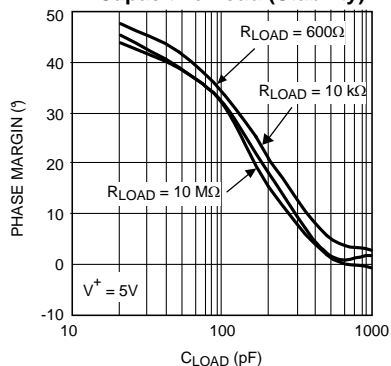
Capacitive Load (Stability)
