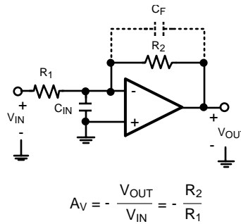
Figure 6. Inverting Amplifier
