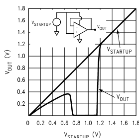
Figure 7. Output Voltage vs. Supply Voltage
