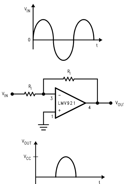
Figure 8. Half-Wave Rectifier with Rail-To-Ground Output Swing Referenced to Ground
