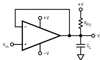
Figure 4. Using a Pull-Up Resistor at the Output for Stabilizing Capacitive Loads
