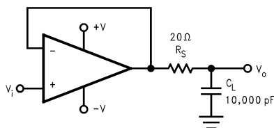
Figure 5. Using an Isolation Resistor to Drive Heavy Capacitive Loads
