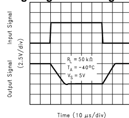
*Large Signal Non-Inverting Response
