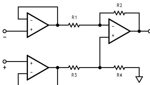
Figure 10. Rail-to-rail instrumentation amplifier
