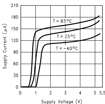
Figure 1. Supply Current vs. Supply Voltage (LMV921)
