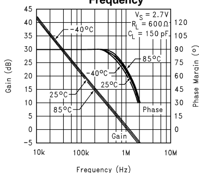
Gain and Phase Margin vs. Frequency
