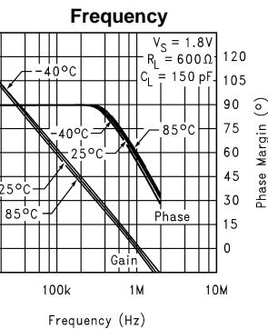
Gain and Phase Margin vs. Frequency
