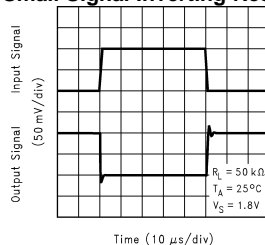
Small Signal Inverting Response
