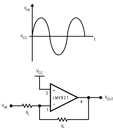
Figure 8. Half-Wave Rectifier with Rail-To-Ground Output Swing Referenced to Ground
