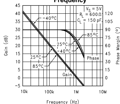
Gain and Phase Margin vs. Frequency
