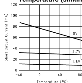
Temperature (sinking)
