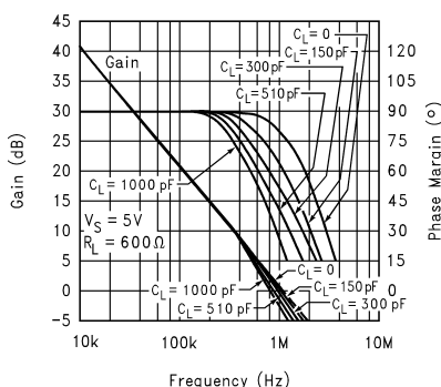
Figure 3. Gain and Phase Margin vs. Frequency
