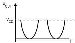
Figure 9. Half-Wave Rectifier with Negative-Going Output Referenced to V_{CC}
