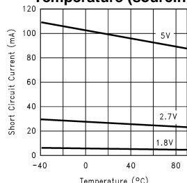
Temperature (sourcing)
