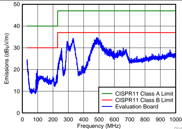
Figure 7. Radiated EMI
