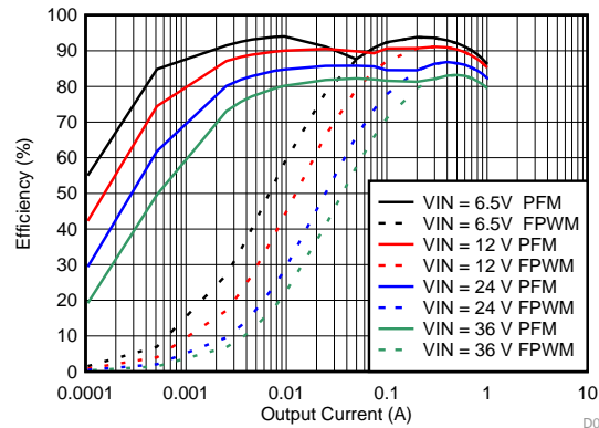
Figure 34. Efficiency
