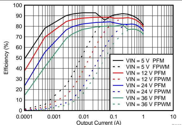
Figure 40. Efficiency
