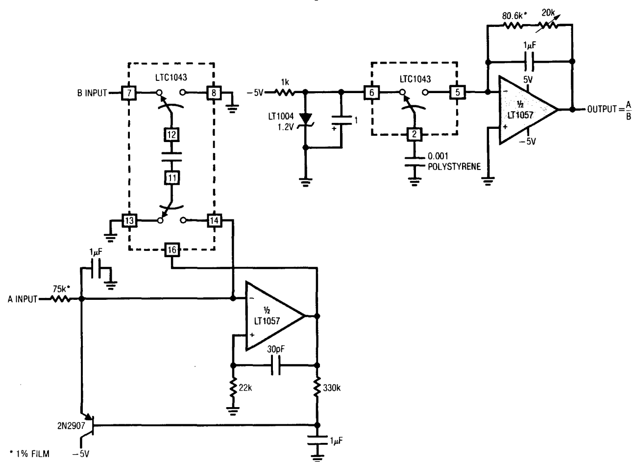
Analog Divider
