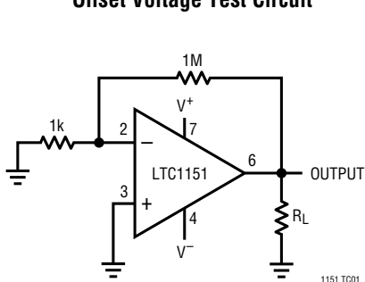
Offset Voltage Test Circuit
