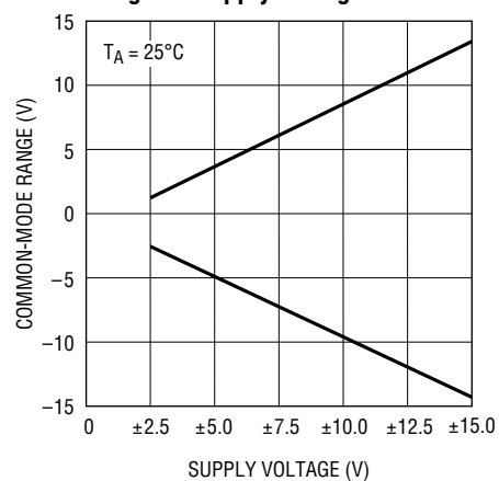
Common-Mode Input Voltage Range vs Supply Voltage
