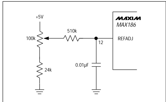
Figure 17. MAX186 Reference-Adjust Circuit
