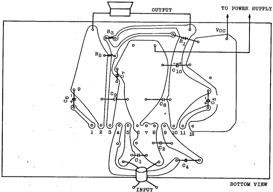
PRINT BOARD (BTL MODE)
