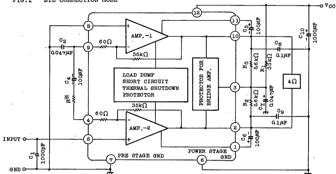
FIG.2 BTL CONNECTION MODE
