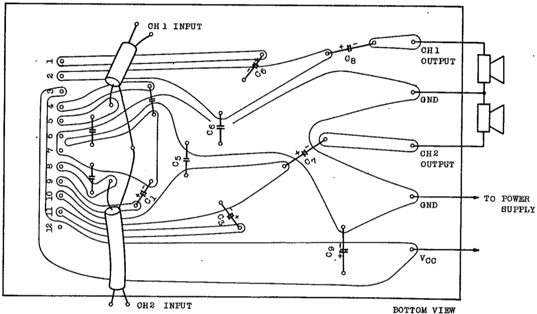
PRINT BOARD (BTL MODE)
