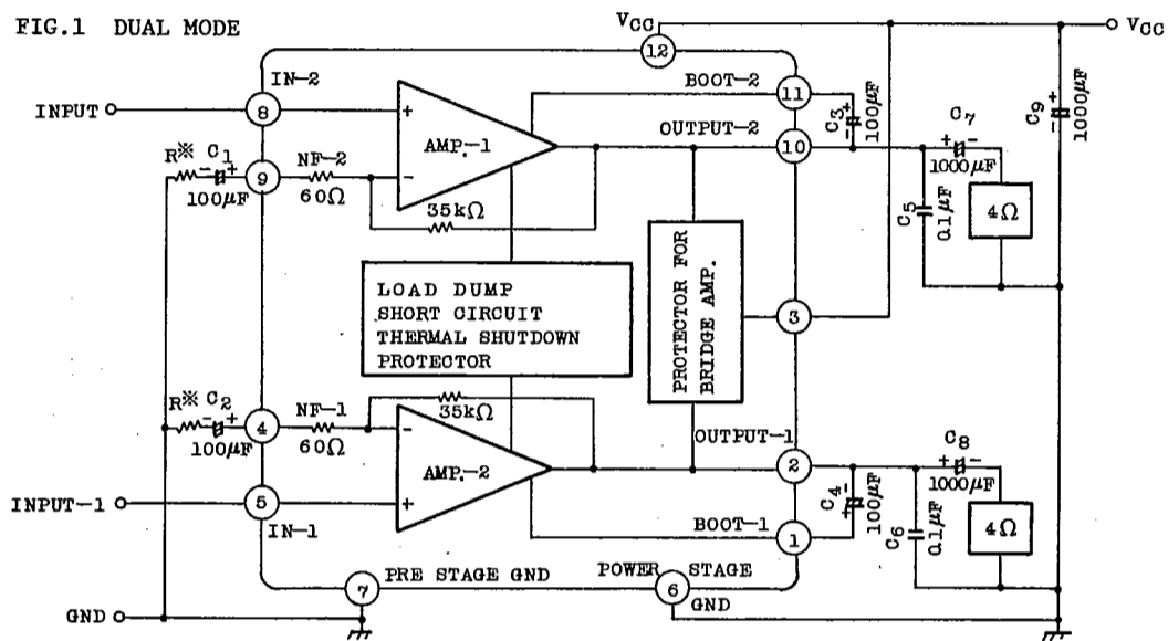
TEST CIRCUIT
