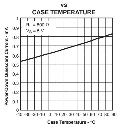
POWER-DOWN QUIESCENT CURRENT
