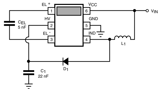
FIGURE 1: TYPICAL APPLICATION
