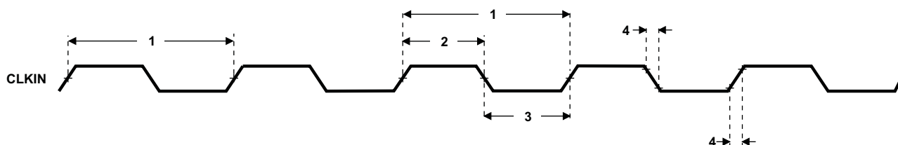
Figure 6-9. CLKIN Timing
